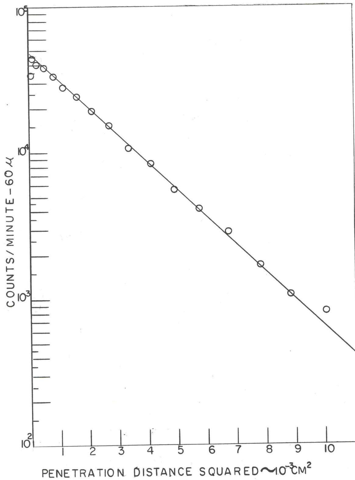
Figure 6. Solute Penetration Curve, Sample No. 72-- Annealed at 24 kb. pressure and 625°K for 4.4 \times 10^4 sec
